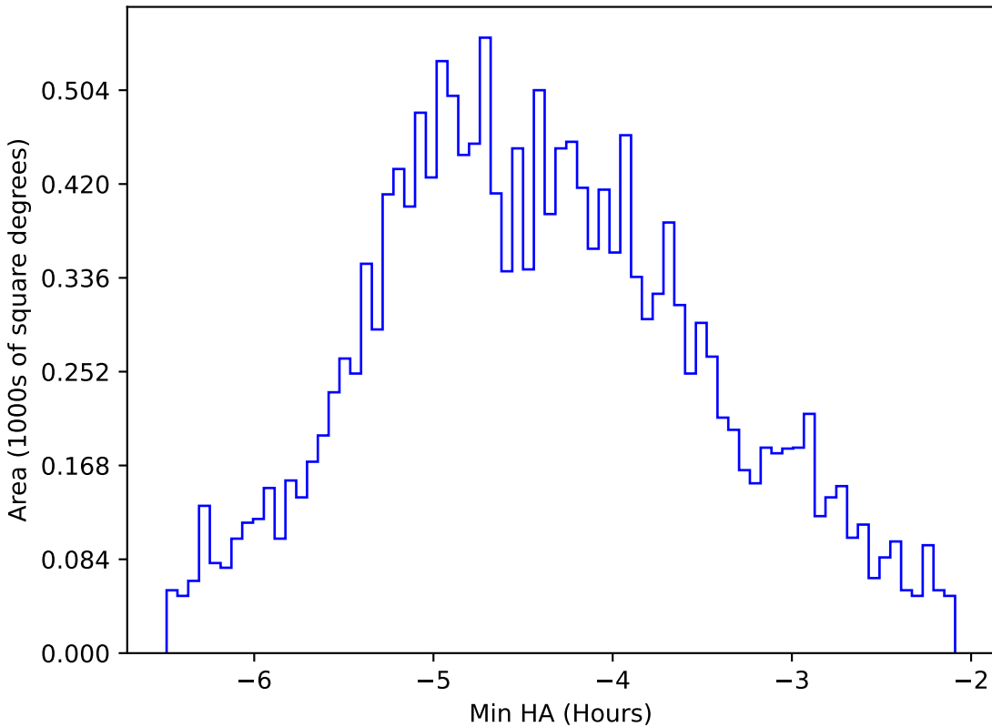
ddf_acor_sf25_lsf40_lsr20_v3.4_10yrs WFD z band: Min HA
