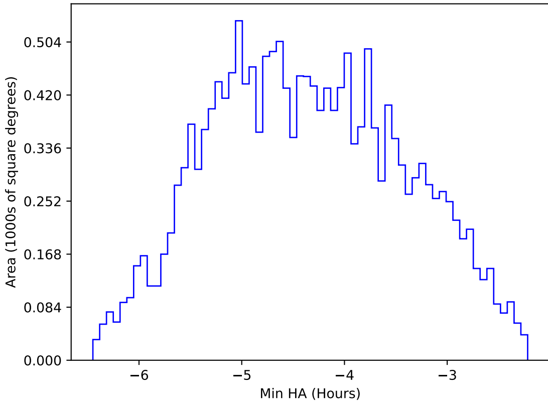
ddf_acor_sf25_lsf40_lsr20_v3.4_10yrs WFD i band: Min HA
