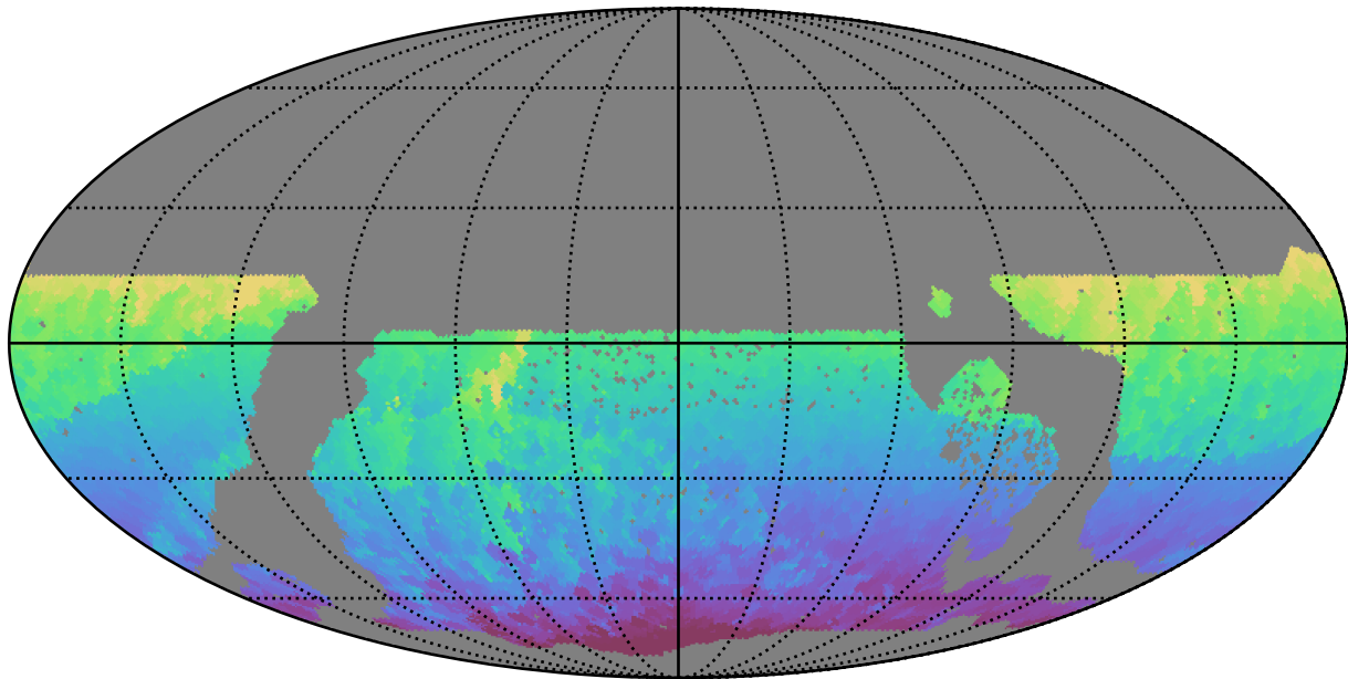
ddf_acor_sf25_lsf40_lsr20_v3.4_10yrs WFD all bands: Min HA
