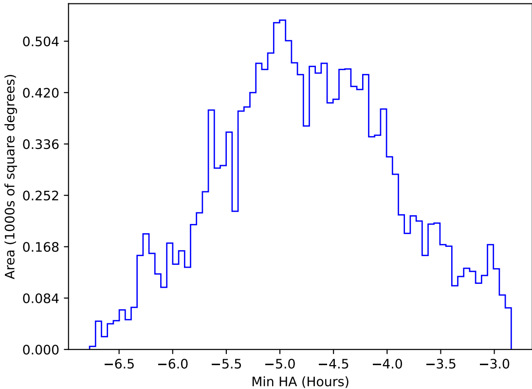
ddf_acor_sf25_lsf40_lsr20_v3.4_10yrs WFD all bands: Min HA
