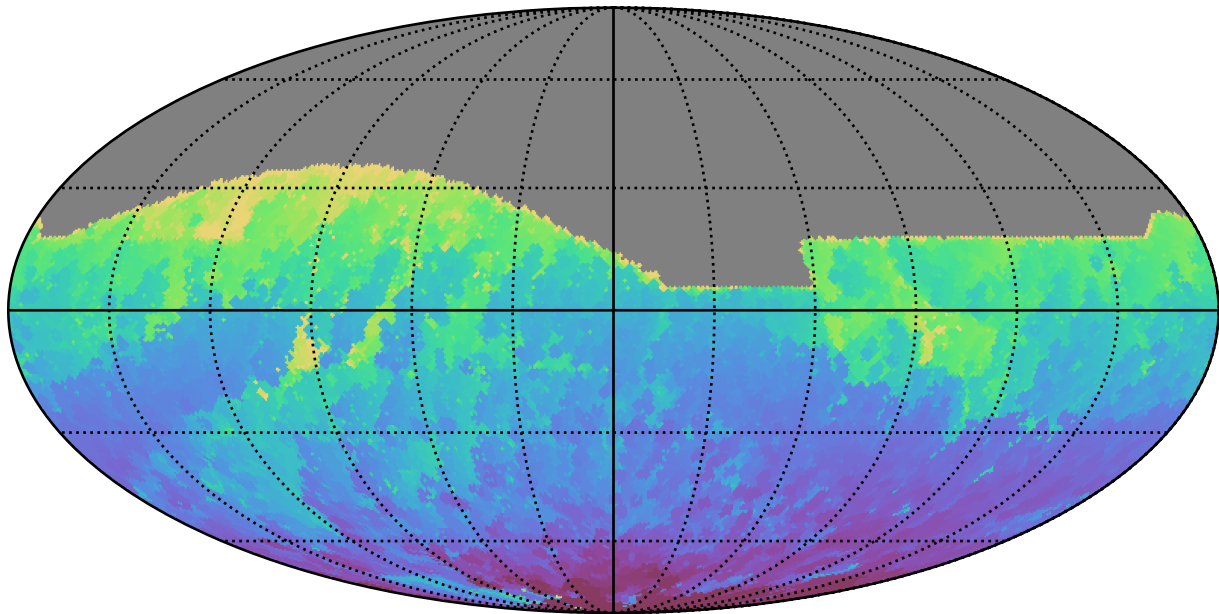
ddf_acor_sf25_lsf40_lsr20_v3.4_10yrs All sky z band: Min HA
