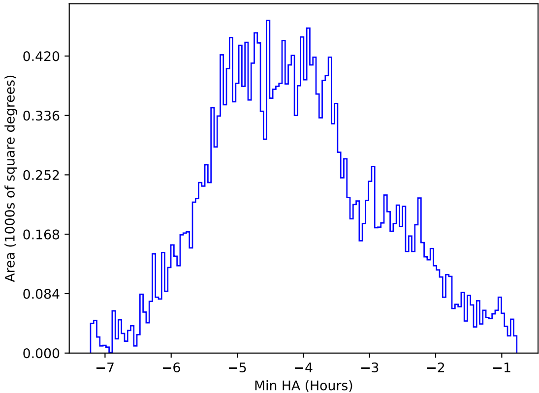
ddf_acor_sf25_ls40_lsr20_v3.4_10yrs All sky z band: Min HA
