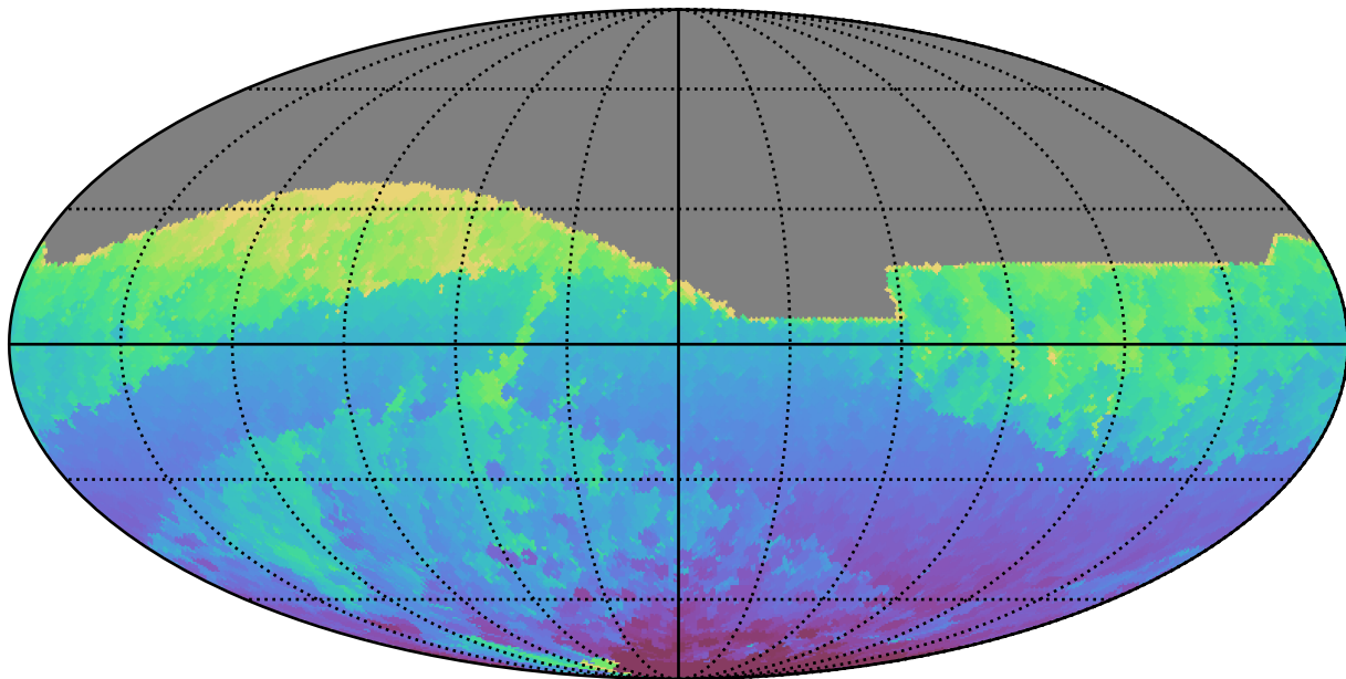
ddf_acor_sf25_lsf40_lsr20_v3.4_10yrs All sky r band: Min HA
