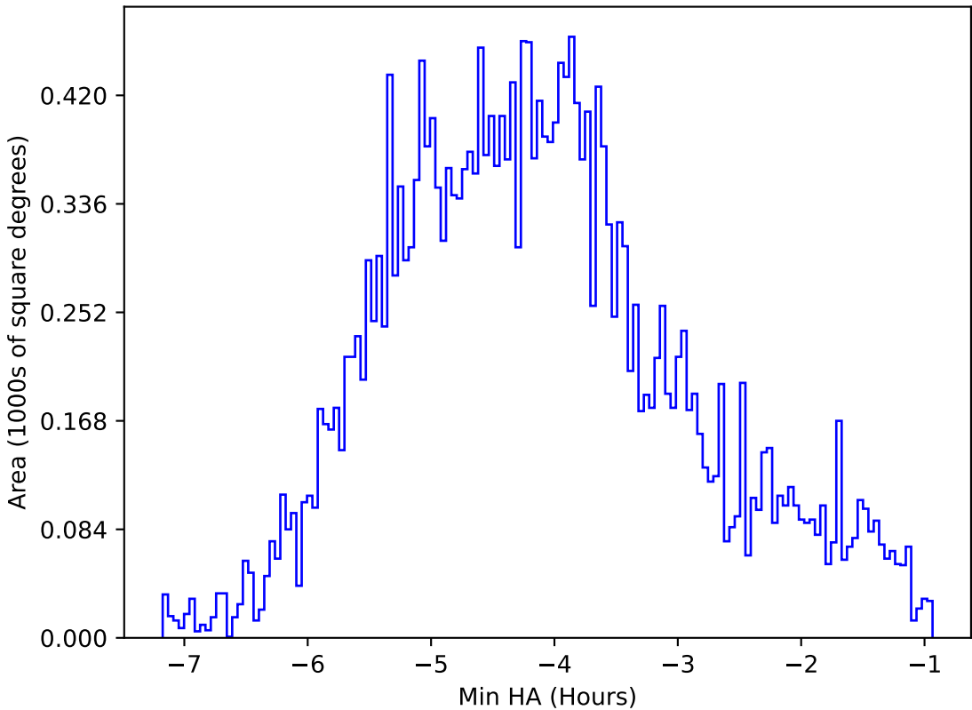
ddf_acor_sf25_ls40_lsr20_v3.4_10yrs All sky r band: Min HA
