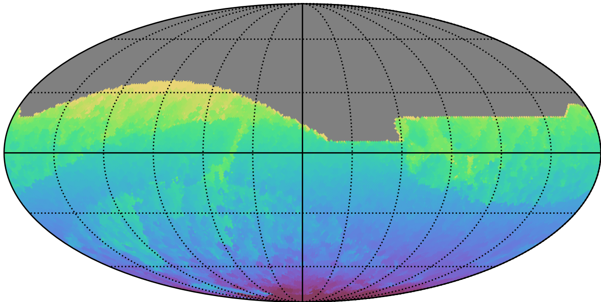
ddf_acor_sf25_lsf40_lsr20_v3.4_10yrs All sky all bands: Min HA
