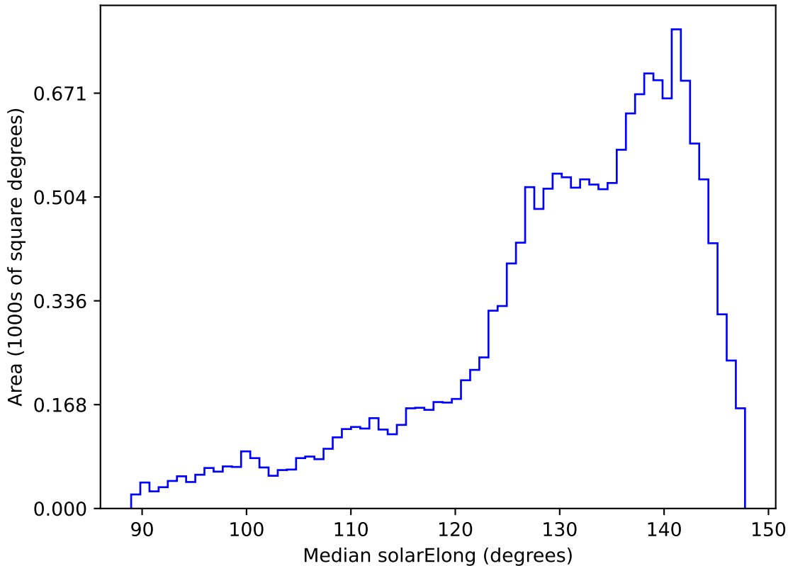
ddf_acor_sf25_lsf40_lsr20_v3.4_10yrs WFD y band: Median solarElong
