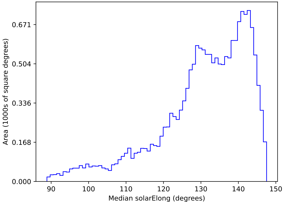
ddf_acor_sf25_lsf40_lsr20_v3.4_10yrs WFD r band: Median solarElong
