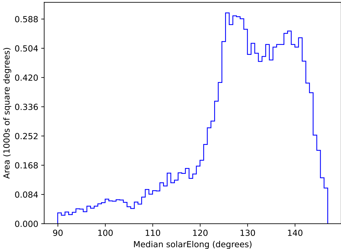
ddf_acor_sf25_lsf40_lsr20_v3.4_10yrs WFD i band: Median solarElong
