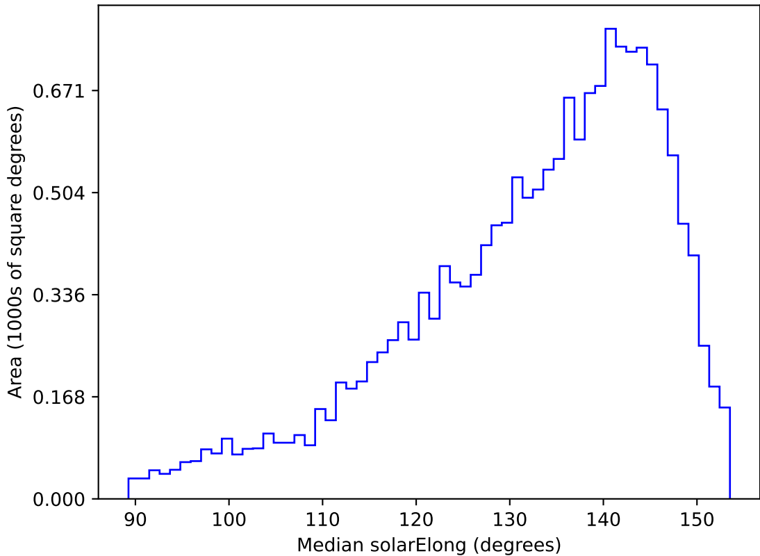
ddf_acor_sf25_lsf40_lsr20_v3.4_10yrs WFD g band: Median solarElong
