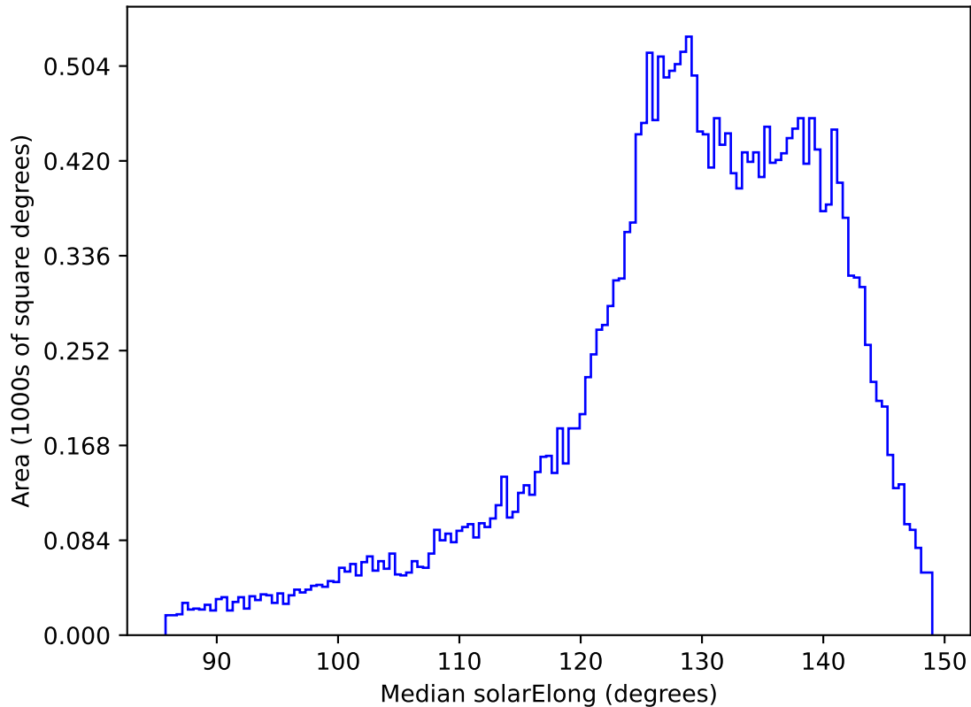
ddf_acor_sf25_lsf40_lsr20_v3.4_10yrs All sky i band: Median solarElong
