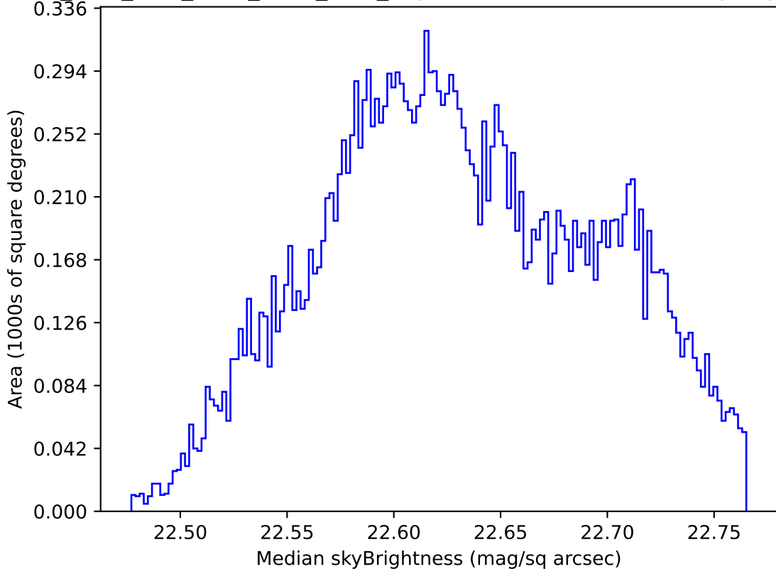
ddf_acor_sf25_Isf40_Isr20_v3.4_10yrs Yr 1 u band: Median skyBrightness
