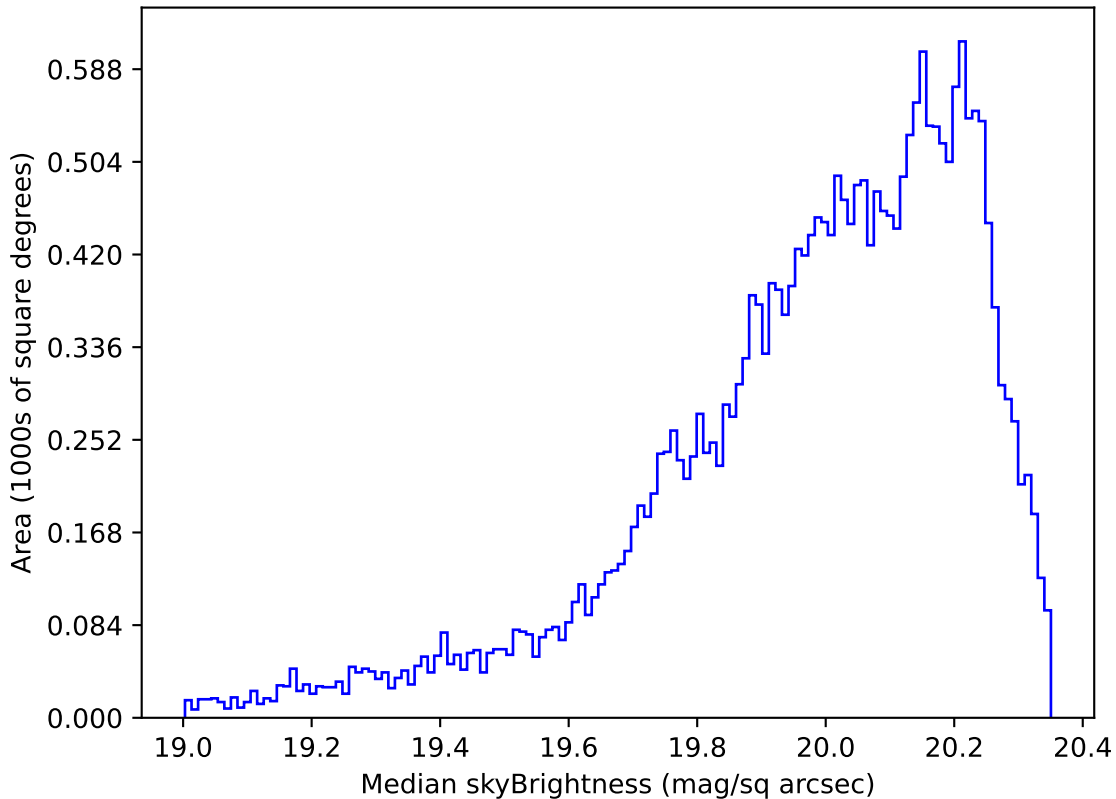
ddf_acor_sf25_lsf40_lsr20_v3.4_10yrs Yr 1 i band: Median skyBrightness
