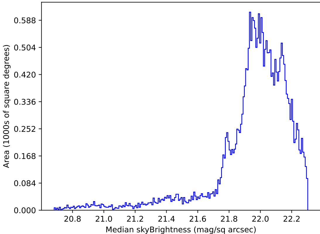
ddf_acor_sf25_lsf40_lsr20_v3.4_10yrs Yr 1 g band: Median skyBrightness
