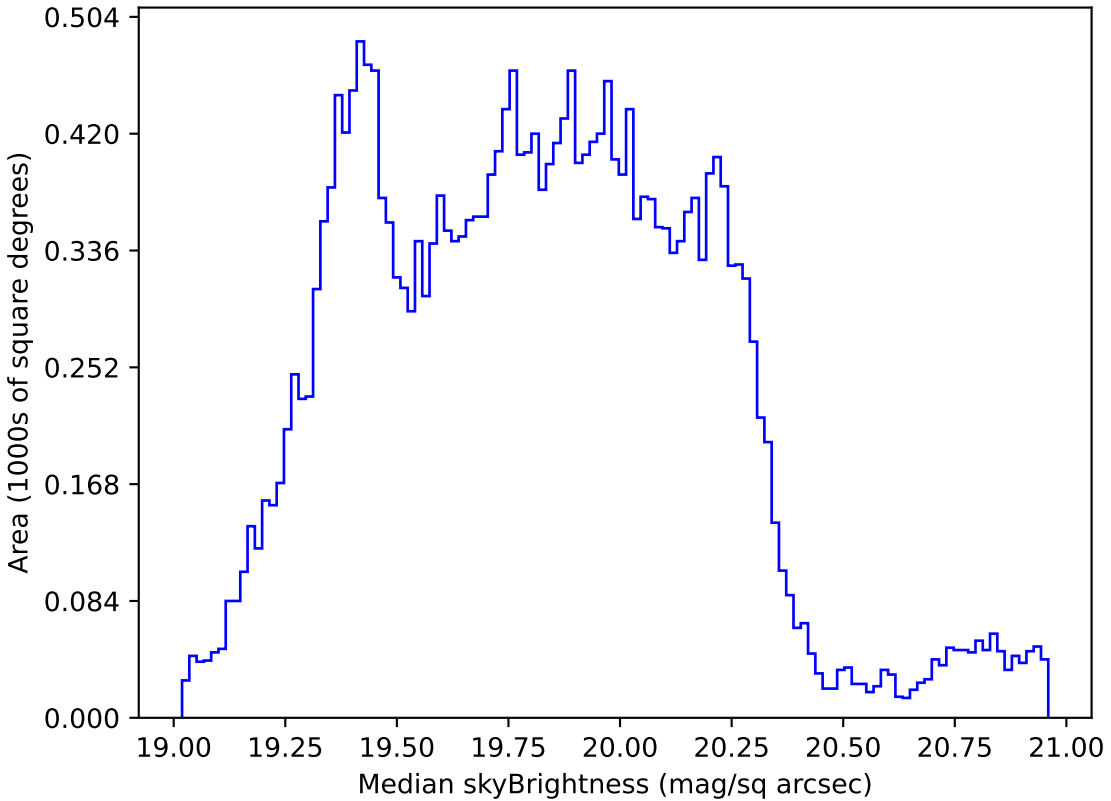
ddf_acor_sf25_lsf40_lsr20_v3.4_10yrs Yr 1 all bands: Median skyBrightness
