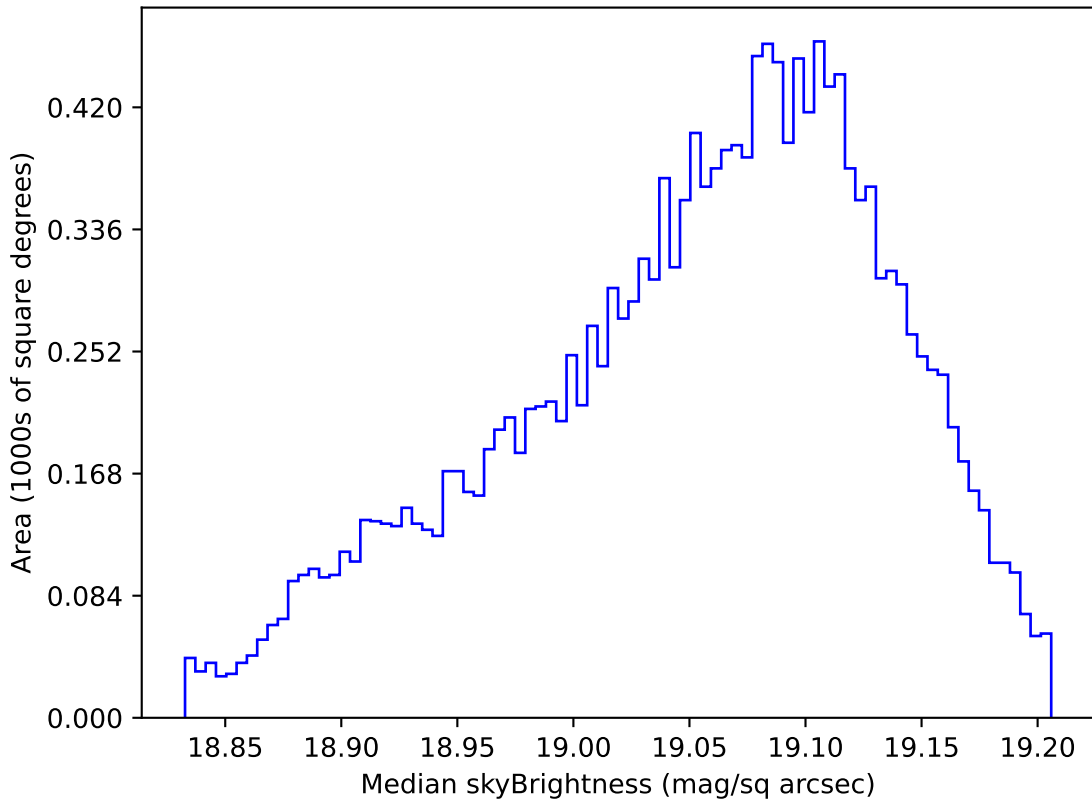
ddf_acor_sf25_lsf40_lsr20_v3.4_10yrs WFD z band: Median skyBrightness
