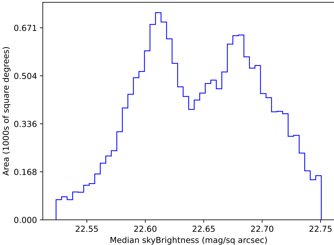
ddf_acor_sf25_lsf40_lsr20_v3.4_10yrs WFD u band: Median skyBrightness
