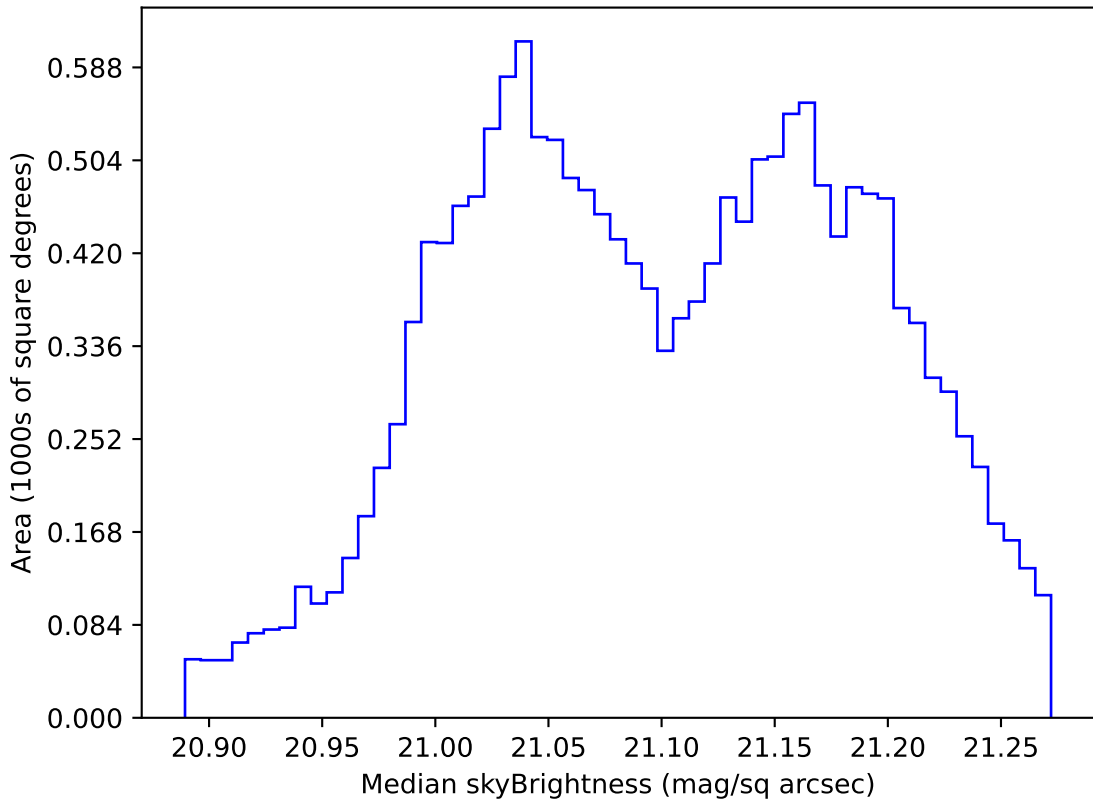
ddf_acor_sf25_lsf40_lsr20_v3.4_10yrs WFD r band: Median skyBrightness
