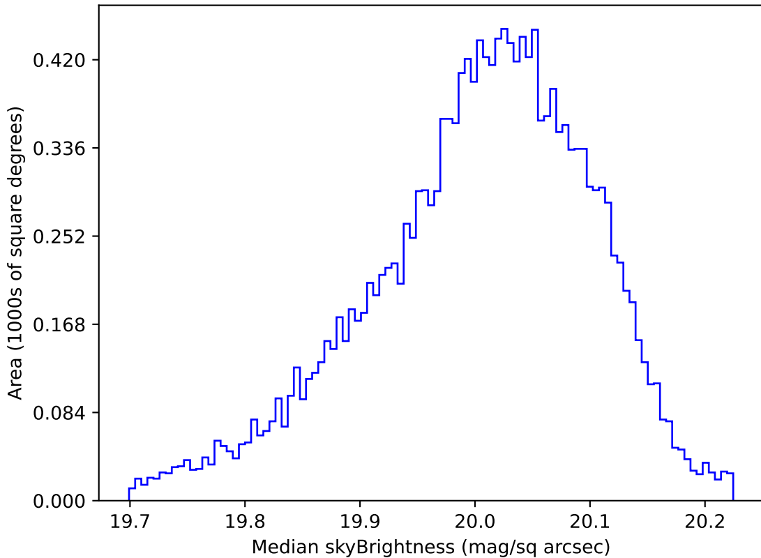
ddf_acor_sf25_lsf40_lsr20_v3.4_10yrs WFD i band: Median skyBrightness
