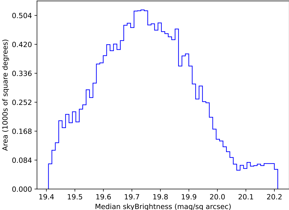
ddf_acor_sf25_lsf40_lsr20_v3.4_10yrs WFD all bands: Median skyBrightness
