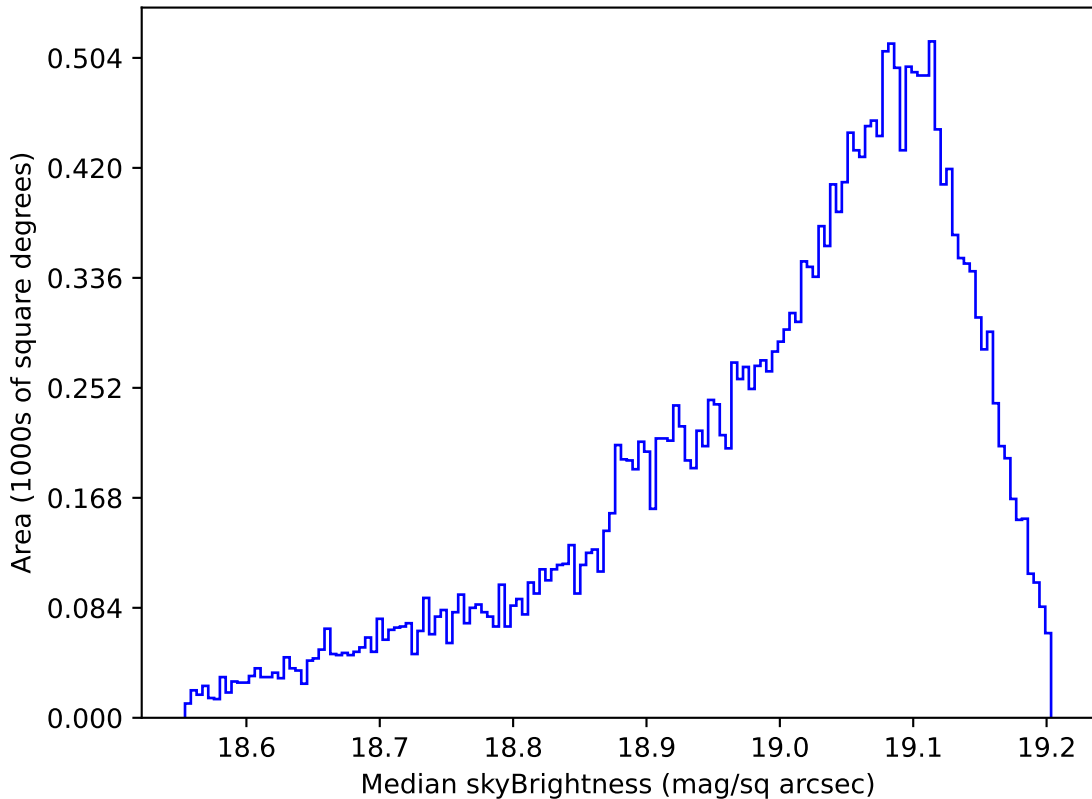
ddf_acor_sf25_lsf40_lsr20_v3.4_10yrs All sky z band: Median skyBrightness
