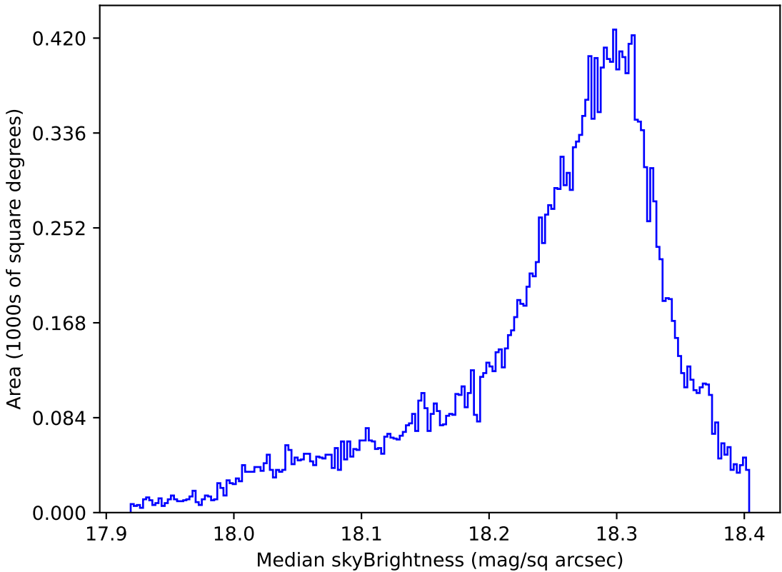
ddf_acor_sf25_lsf40_lsr20_v3.4_10yrs All sky y band: Median skyBrightness
