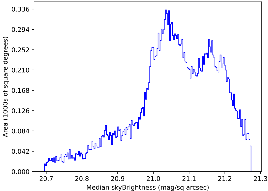
ddf_acor_sf25_lsf40_lsr20_v3.4_10yrs All sky r band: Median skyBrightness
