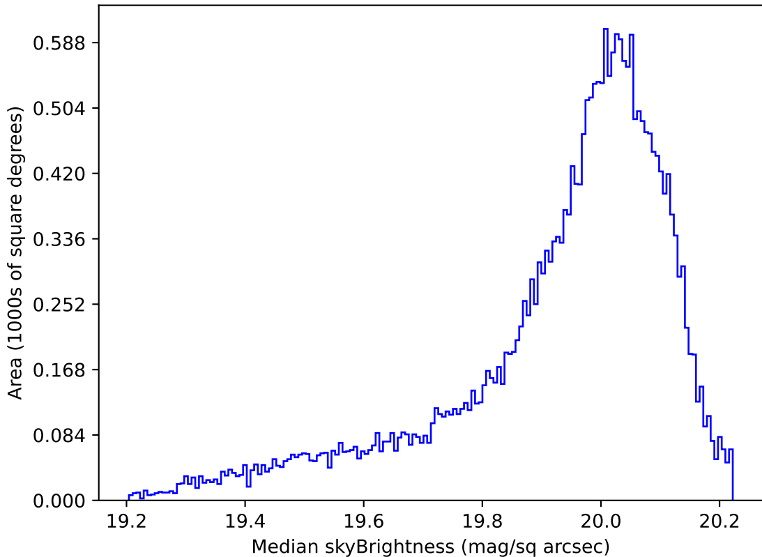
ddf_acor_sf25_lsf40_lsr20_v3.4_10yrs All sky i band: Median skyBrightness
