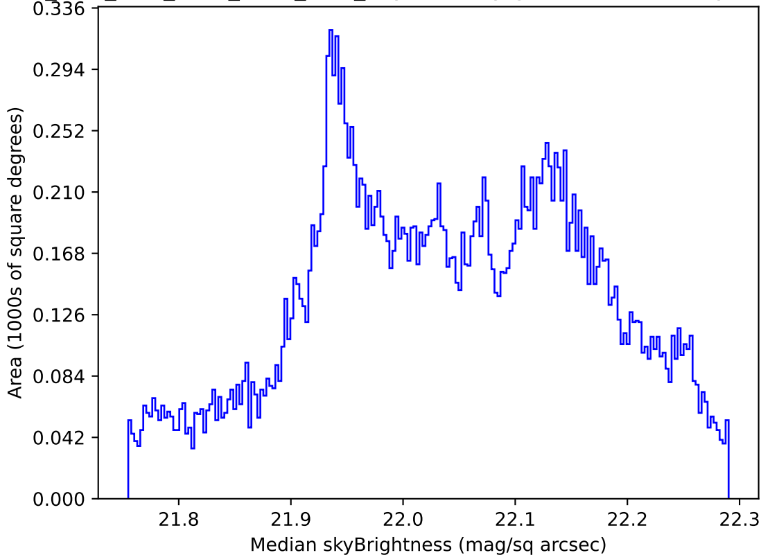
ddf_acor_sf25_lsf40_lsr20_v3.4_10yrs All sky g band: Median skyBrightness
