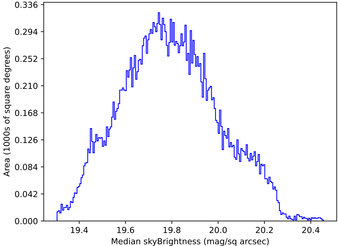
ddf_acor_sf25_lsf40_lsr20_v3.4_10yrs All sky all bands: Median skyBrightness
