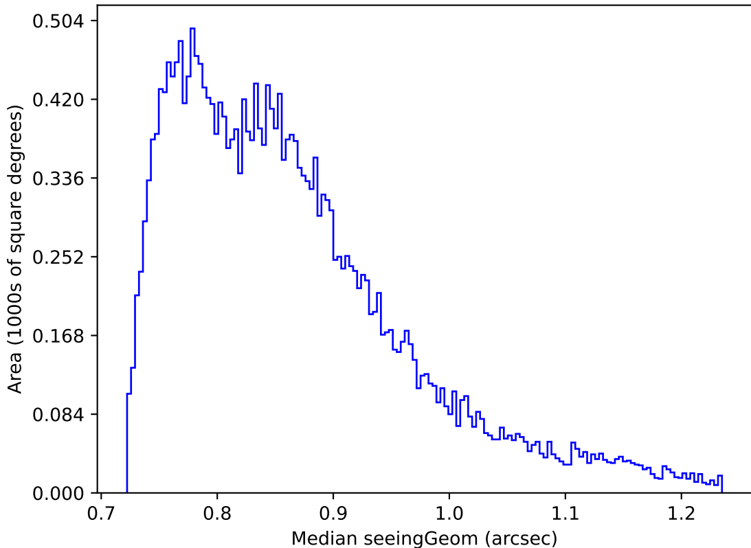
ddf_acor_sf25_lsf40_lsr20_v3.4_10yrs Yr 1 all bands: Median seeingGeom
