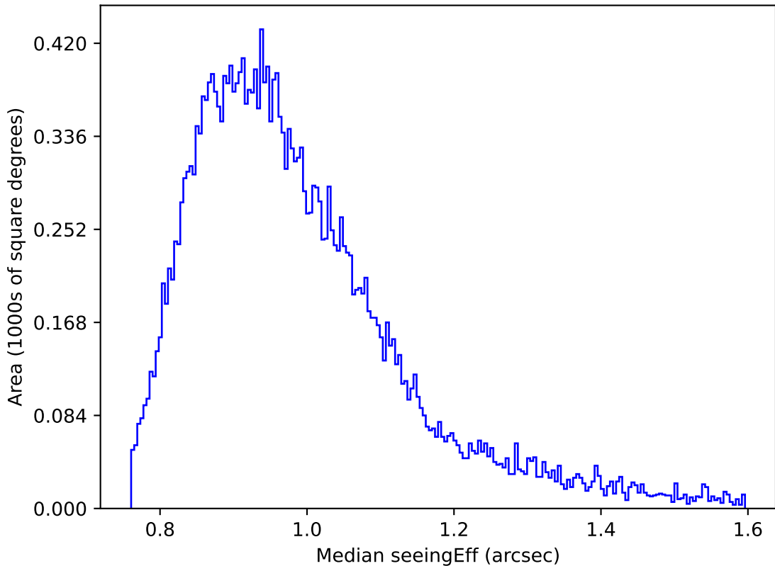
ddf_acor_sf25_lsf40_lsr20_v3.4_10yrs Yr 1 z band: Median seeingEff
