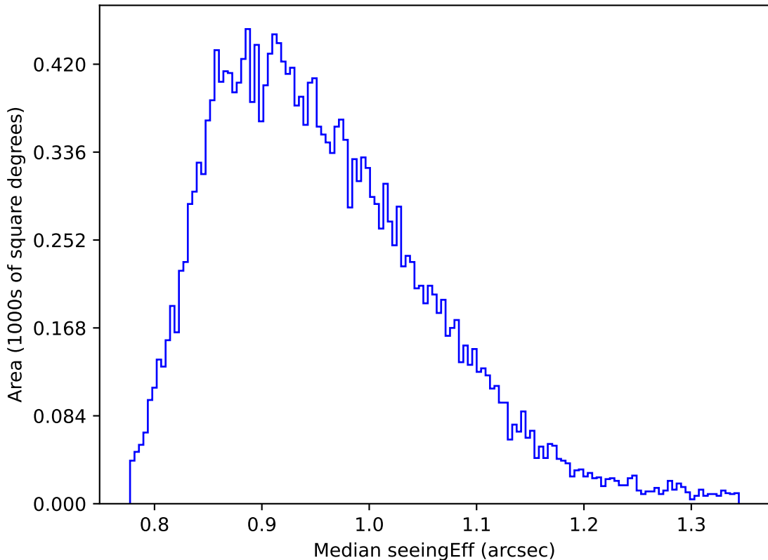
ddf_acor_sf25_lsf40_lsr20_v3.4_10yrs Yr 1 y band: Median seeingEff
