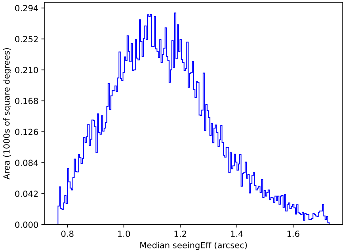
ddf_acor_sf25_lsf40_lsr20_v3.4_10yrs Yr 1 u band: Median seeingEff
