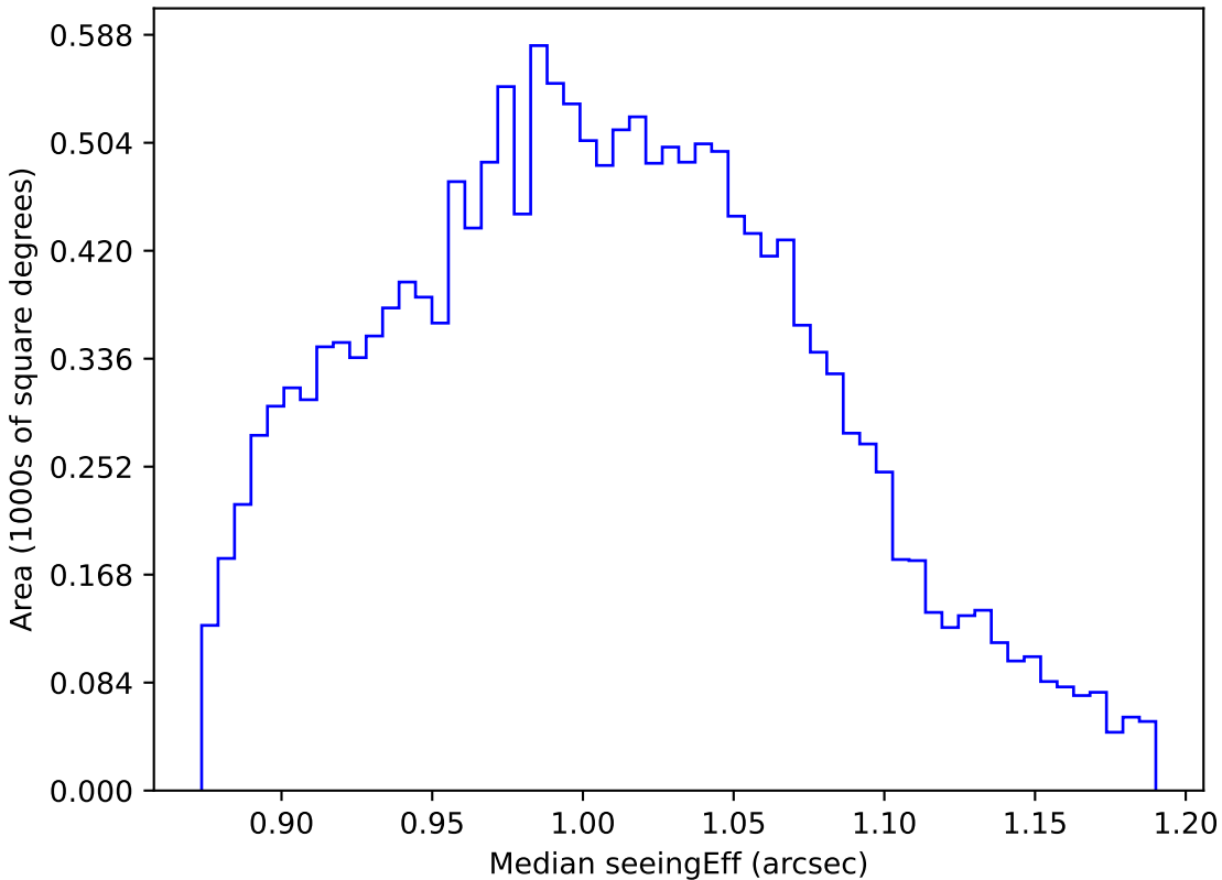
ddf_acor_sf25_lsf40_lsr20_v3.4_10yrs WFD z band: Median seeingEff
