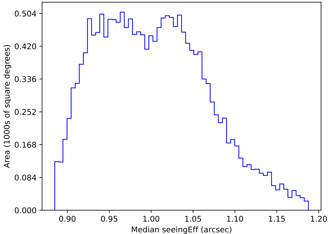
ddf_acor_sf25_lsf40_lsr20_v3.4_10yrs WFD y band: Median seeingEff
