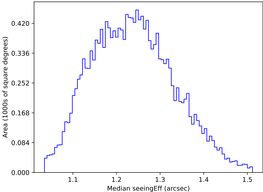
ddf_acor_sf25_lsf40_lsr20_v3.4_10yrs WFD u band: Median seeingEff
