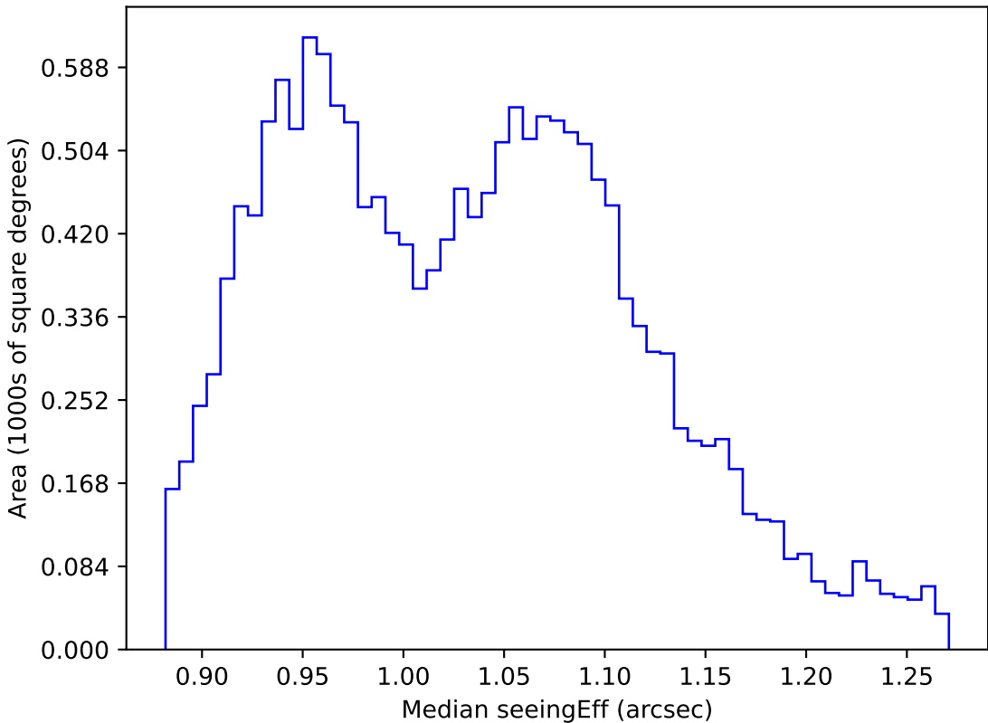
ddf_acor_sf25_lsf40_lsr20_v3.4_10yrs WFD r band: Median seeingEff
