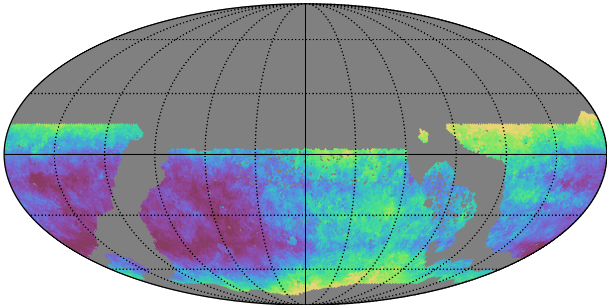
ddf_acor_sf25_lsf40_lsr20_v3.4_10yrs WFD i band: Median seeingEff
