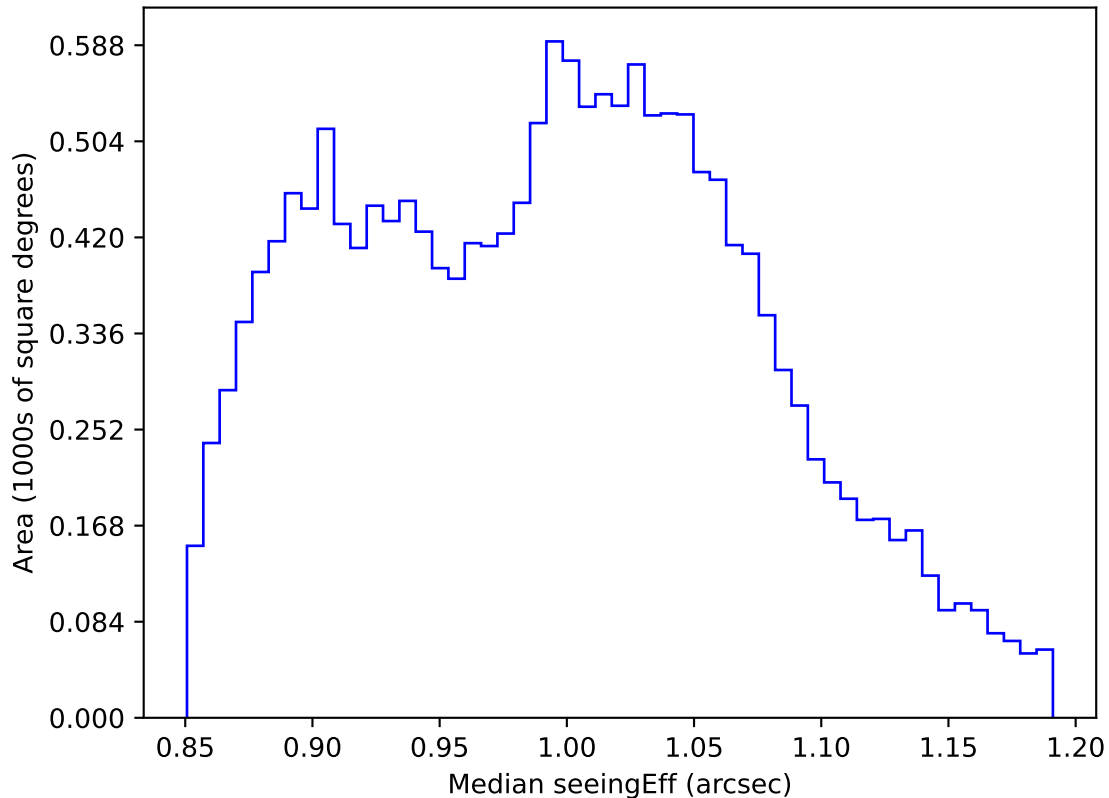
ddf_acor_sf25_lsf40_lsr20_v3.4_10yrs WFD i band: Median seeingEff
