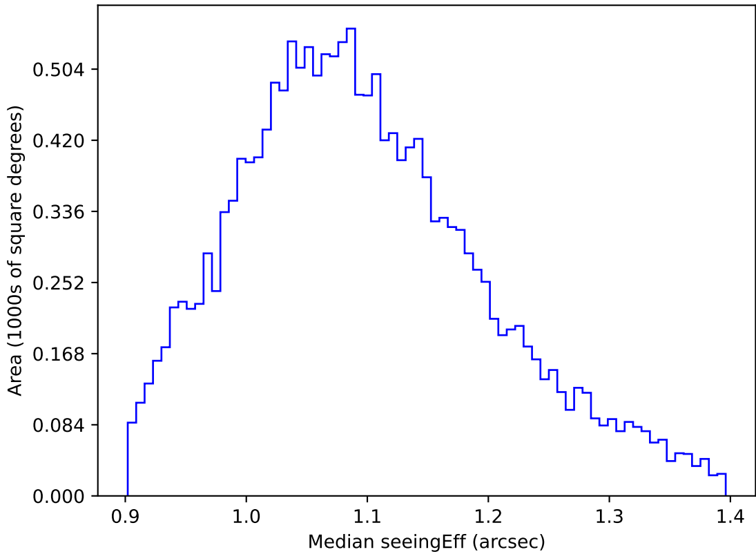
ddf_acor_sf25_lsf40_lsr20_v3.4_10yrs WFD g band: Median seeingEff
