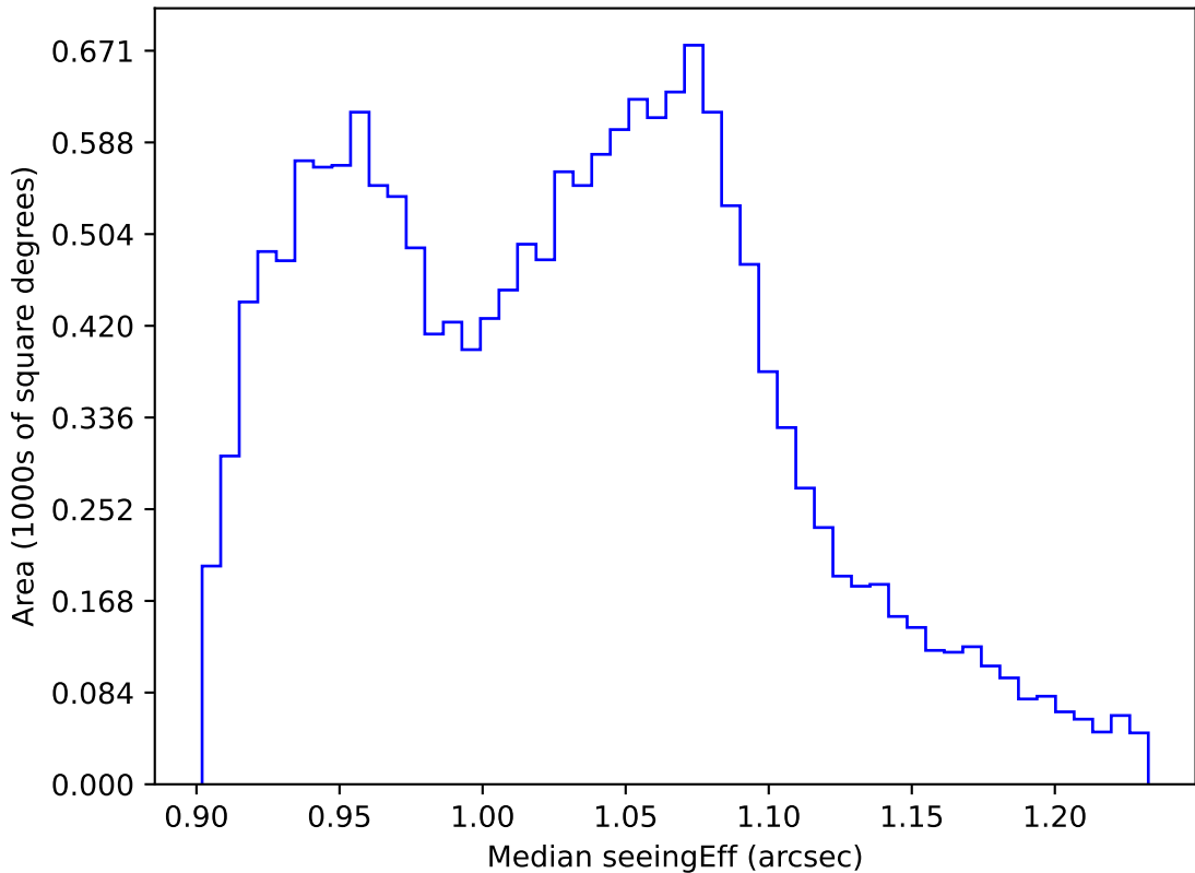
ddf_acor_sf25_lsf40_lsr20_v3.4_10yrs WFD all bands: Median seeingEff
