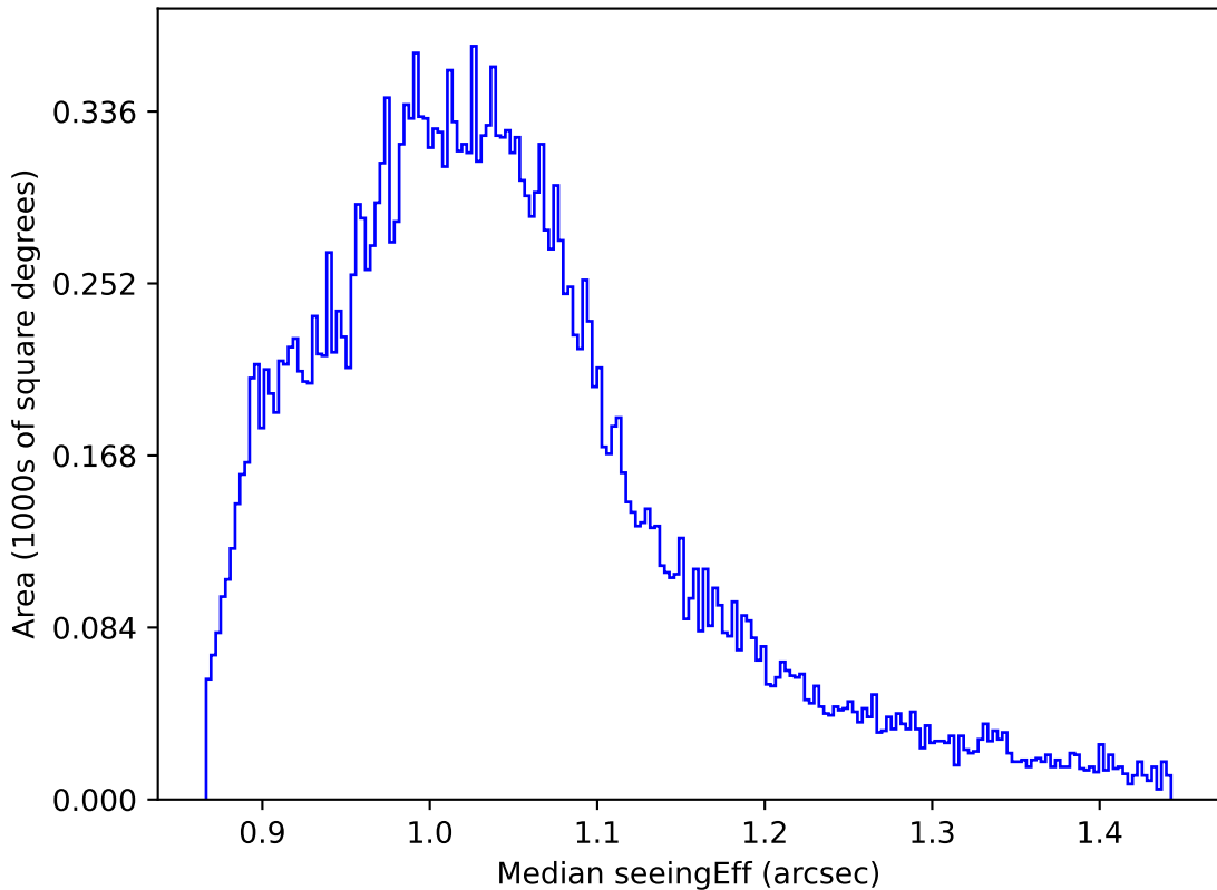
ddf_acor_sf25_lsf40_lsr20_v3.4_10yrs All sky z band: Median seeingEff
