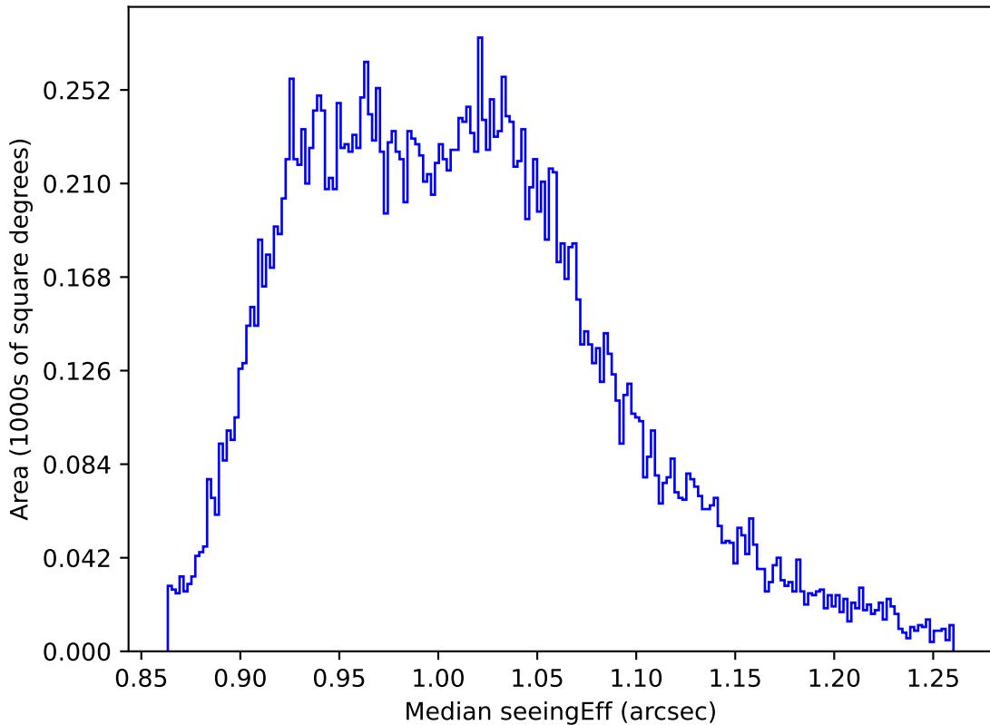
ddf_acor_sf25_ls40_lsr20_v3.4_10yrs All sky y band: Median seeingEff
