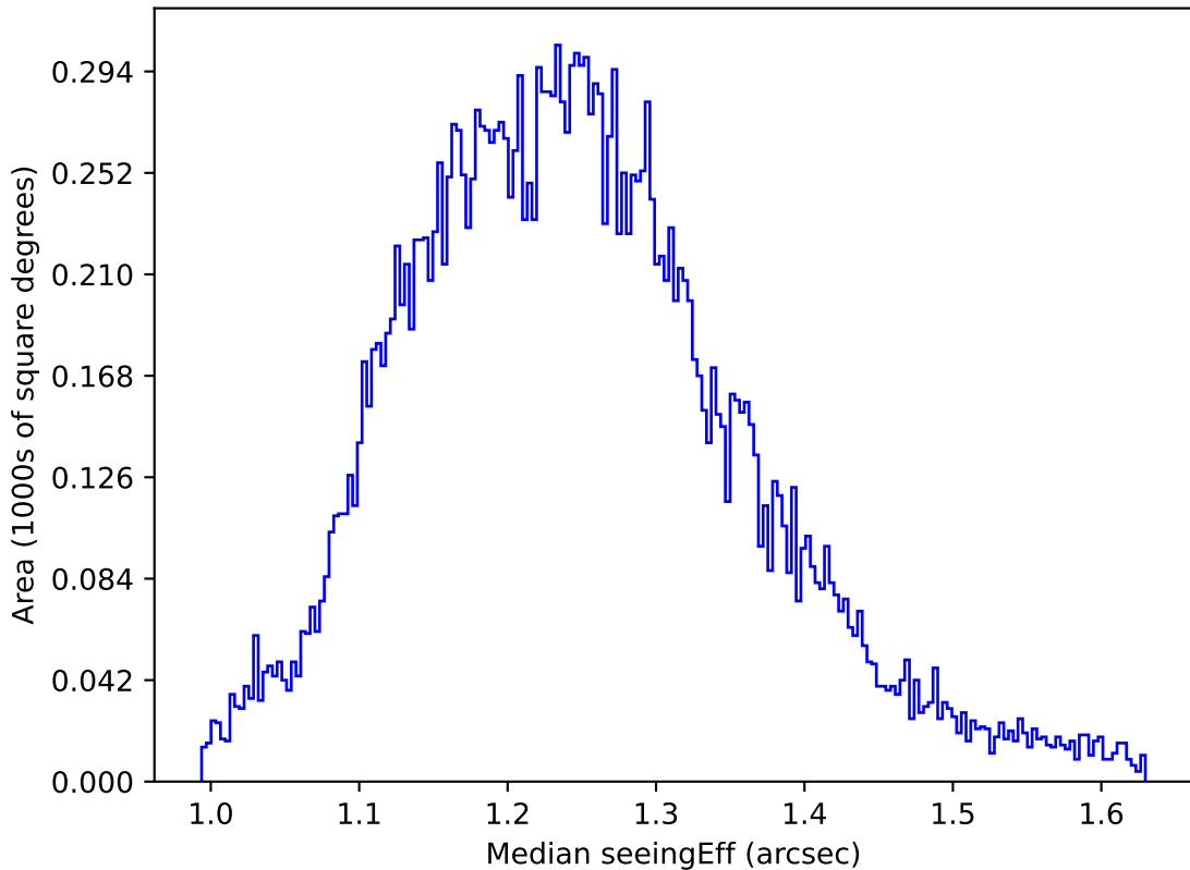
ddf_acor_sf25_lsf40_lsr20_v3.4_10yrs All sky u band: Median seeingEff
