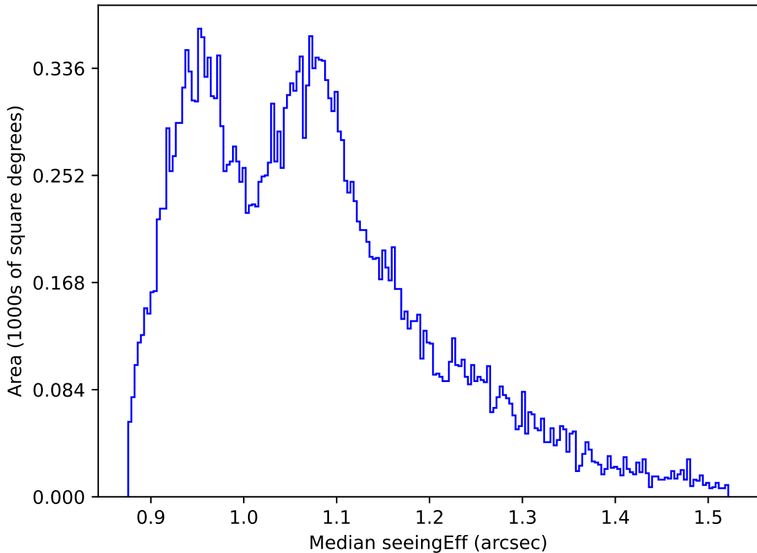
ddf_acor_sf25_lsf40_lsr20_v3.4_10yrs All sky r band: Median seeingEff
