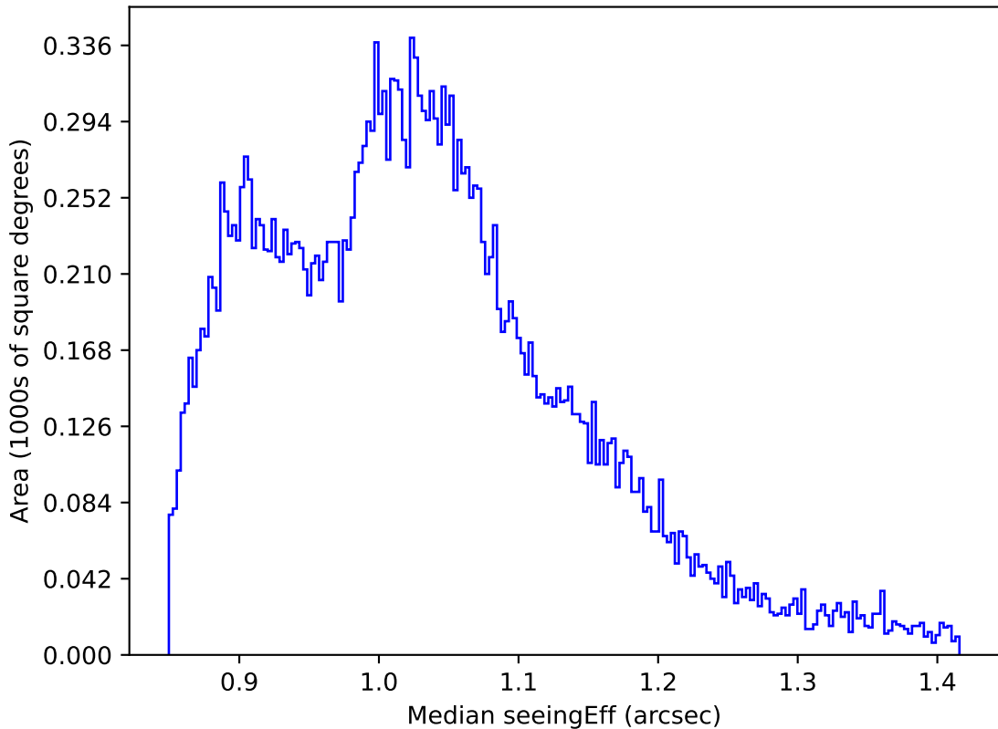
ddf_acor_sf25_lsf40_lsr20_v3.4_10yrs All sky i band: Median seeingEff
