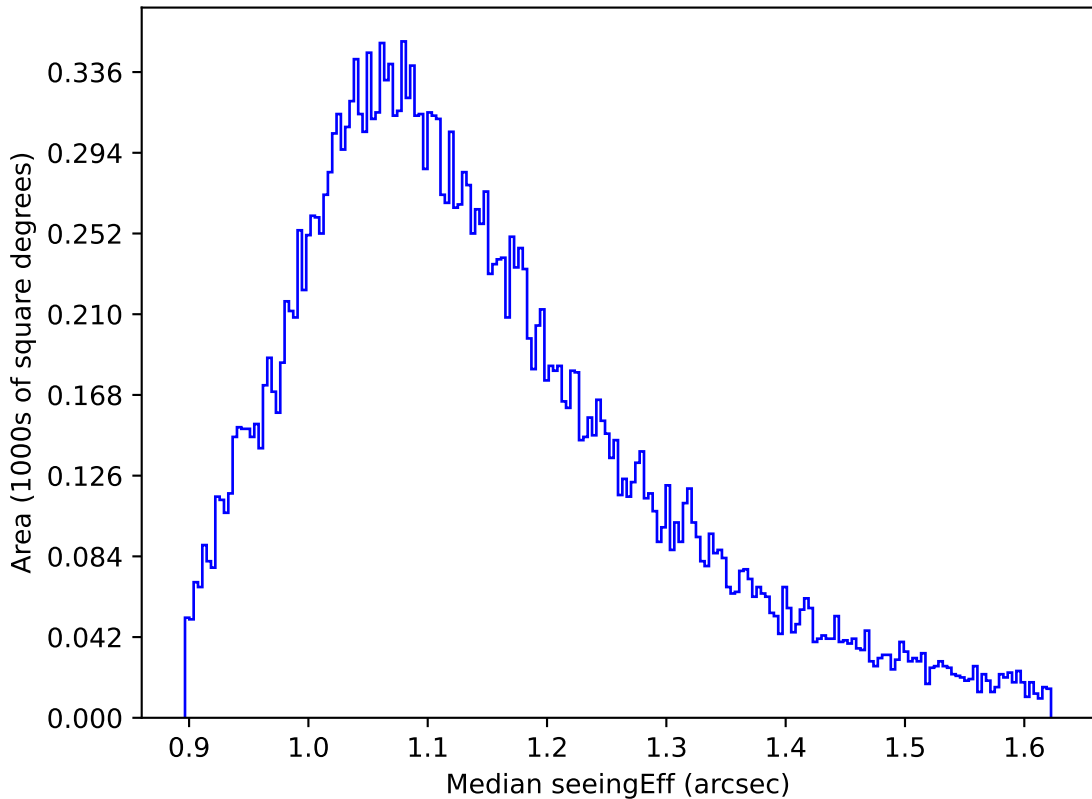
ddf_acor_sf25_lsf40_lsr20_v3.4_10yrs All sky g band: Median seeingEff
