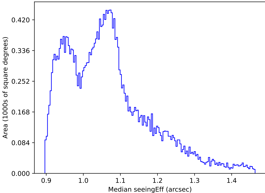
ddf_acor_sf25_lsf40_lsr20_v3.4_10yrs All sky all bands: Median seeingEff
