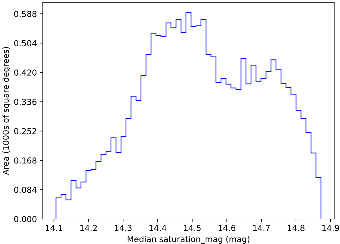
ddf_acor_sf25_lsf40_lsr20_v3.4_10yrs WFD i band: Median saturation_mag
