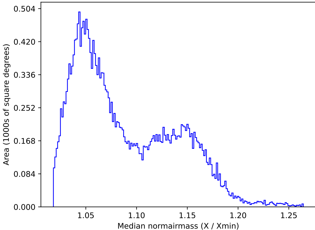
ddf_acor_sf25_lsf40_lsr20_v3.4_10yrs All sky z band: Median normairmass
